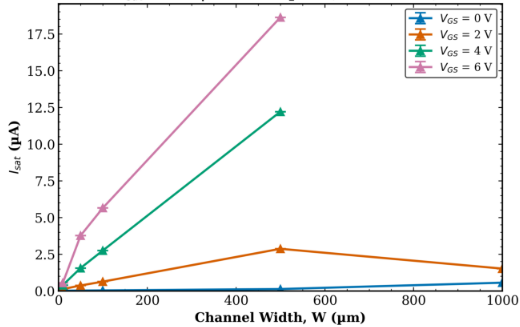
TFT2 Transistor 2 I_{sat} vs W | L = 160 \mu\text{m} (mean \pm std)
