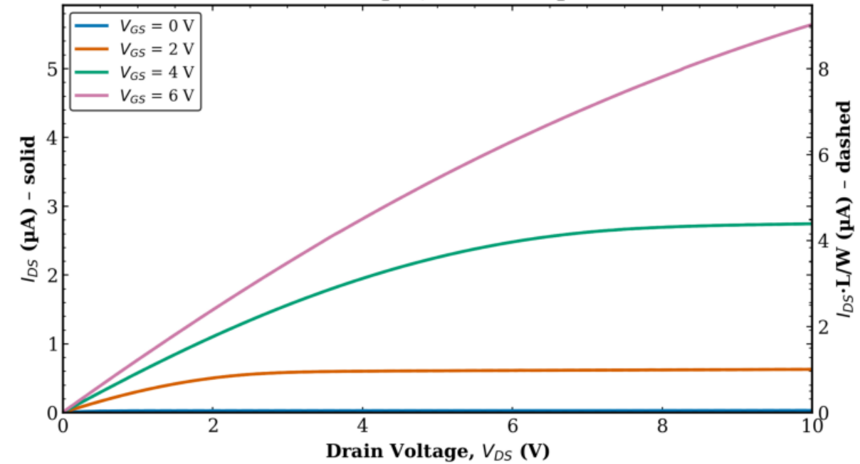
TFT2 Transistor 2 L = 160 \mu\text{m} , W = 100 \mu\text{m}
