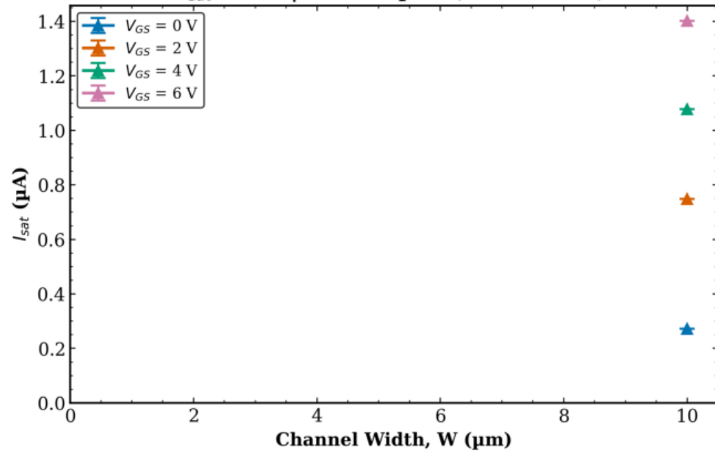
TFT2 Transistor 2 I_{sat} vs W | L = 40 \mu\text{m} (mean \pm std)
