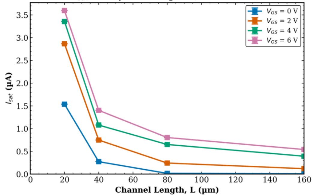
TFT2 Transistor 2 I_{sat} vs L | W = 10 \mu\text{m} (mean \pm std)
