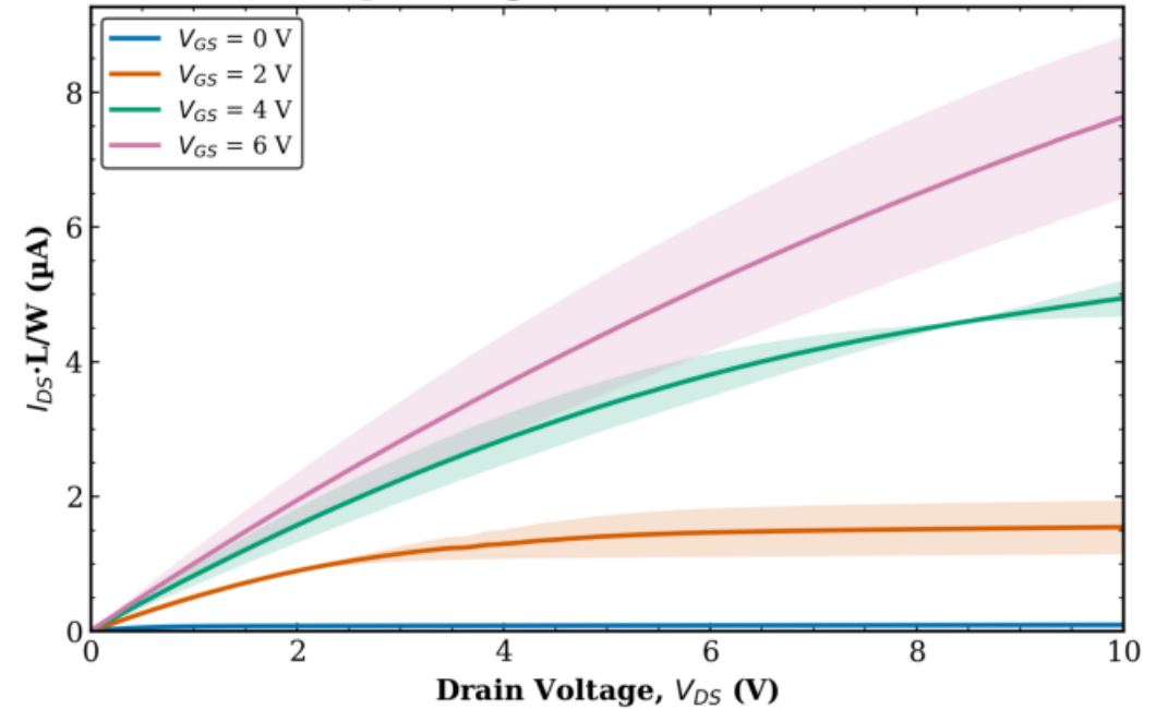
TFT2 Transistor 2 L = 80 \mu\text{m} - avg over all W (mean \pm std)
