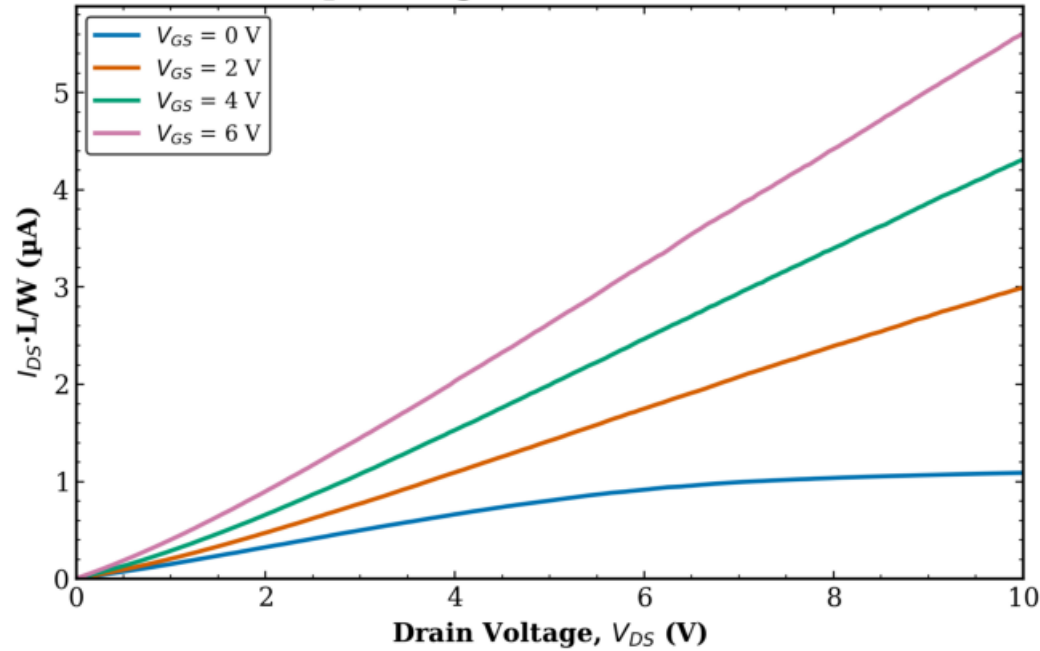
TFT2 Transistor 2 L = 40 \mu\text{m} - avg over all W (mean \pm std)
