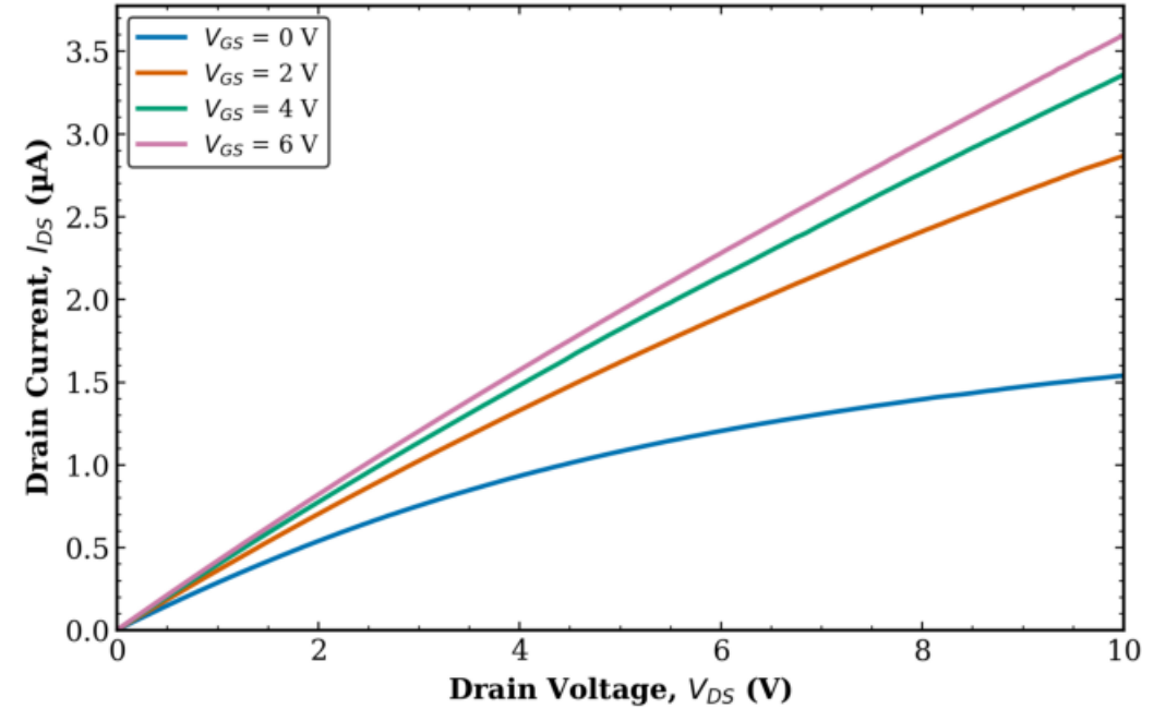
TFT2 Transistor 2 L = 20 \mu\text{m} , W = 10 \mu\text{m}
