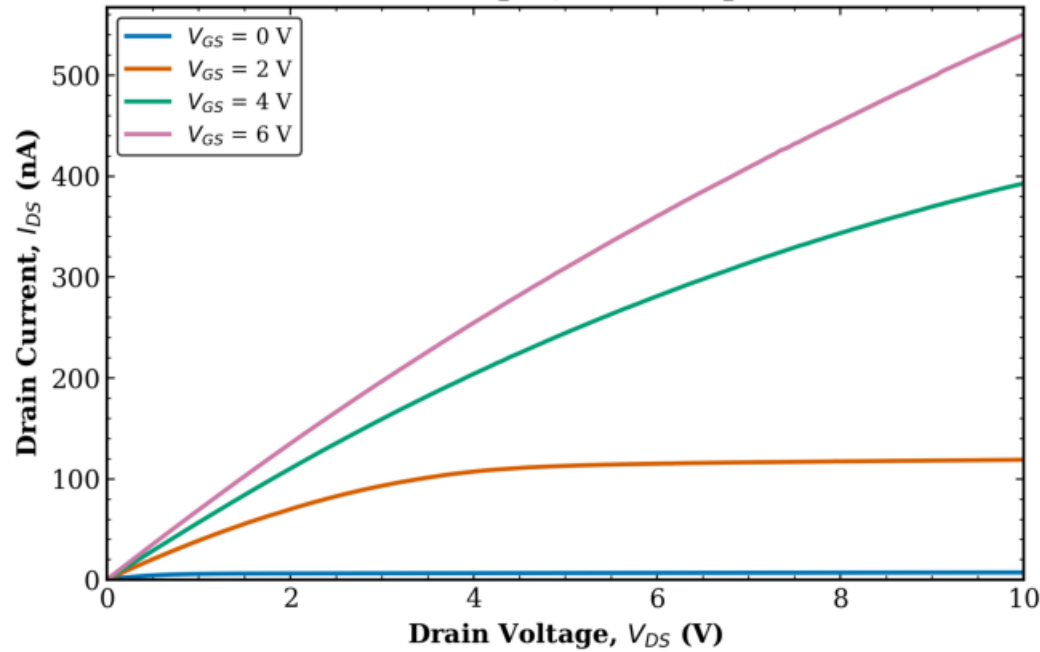
TFT2 Transistor 2 L = 160 \mu\text{m} , W = 10 \mu\text{m}
