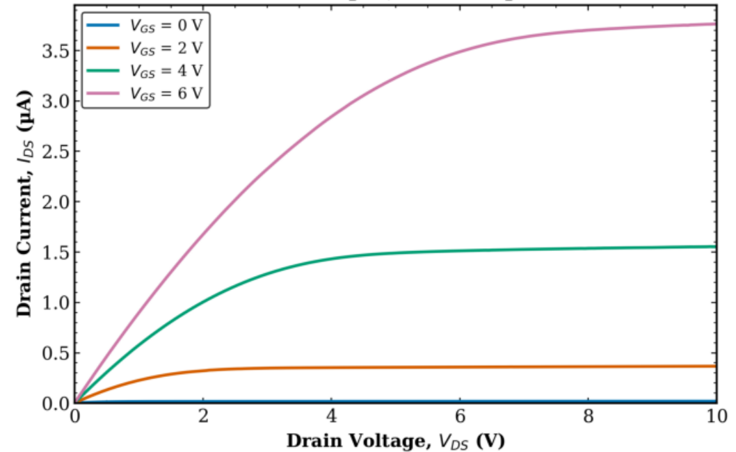
TFT2 Transistor 2 L = 160 \mu\text{m} , W = 50 \mu\text{m}
