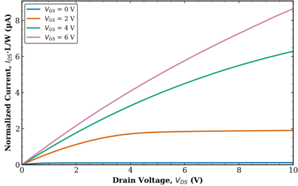
TFT2 Transistor 2 L = 160 \mu\text{m} , W = 10 \mu\text{m} (normalized)
