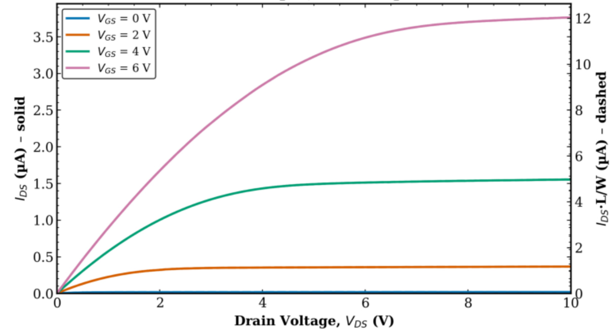
TFT2 Transistor 2 L = 160 \mu\text{m} , W = 50 \mu\text{m}
