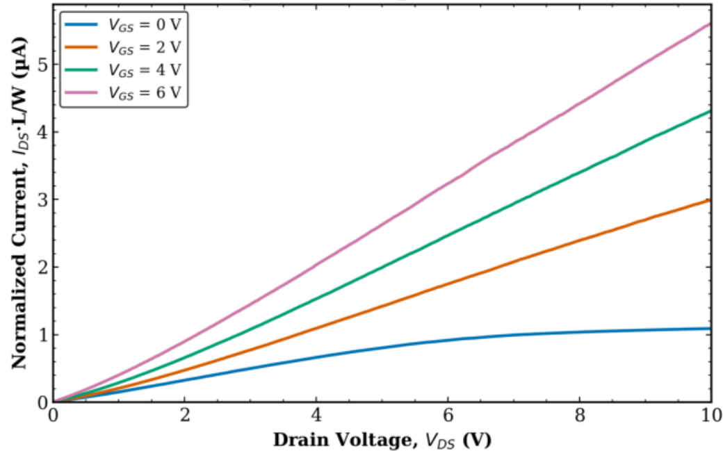
TFT2 Transistor 2 L = 40 \mu\text{m} , W = 10 \mu\text{m} (normalized)
