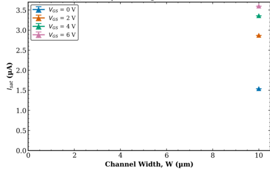
TFT2 Transistor 2 I_{sat} vs W | L = 20 \mu\text{m} (mean \pm std)
