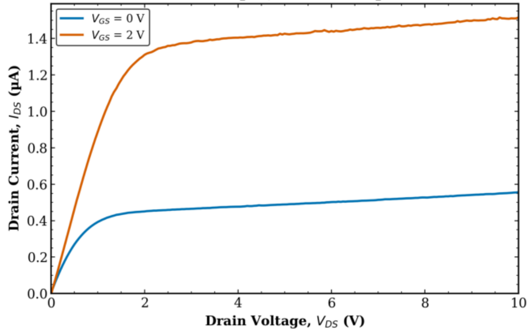
TFT2 Transistor 2 L = 160 \mu\text{m} , W = 1000 \mu\text{m}
