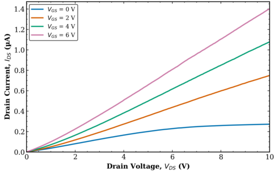
TFT2 Transistor 2 L = 40 \mu\text{m} , W = 10 \mu\text{m}
