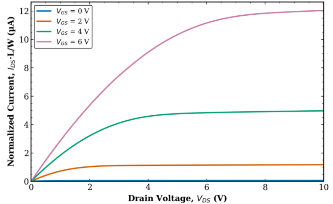
TFT2 Transistor 2 L = 160 \mu\text{m} , W = 50 \mu\text{m} (normalized)
