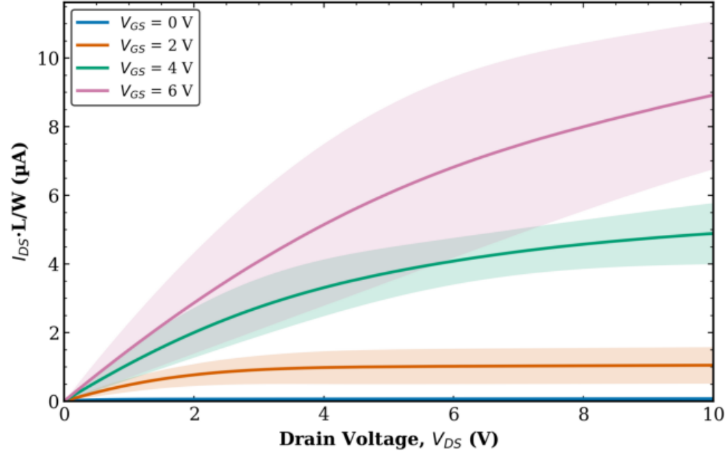
TFT2 Transistor 2 L = 160 \mu\text{m} - avg over all W (mean \pm std)
