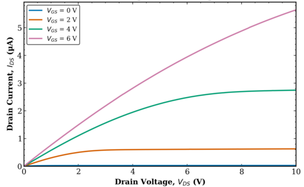
TFT2 Transistor 2 L = 160 \mu\text{m} , W = 100 \mu\text{m}
