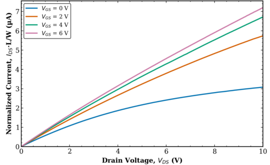
TFT2 Transistor 2 L = 20 \mu\text{m} , W = 10 \mu\text{m} (normalized)
