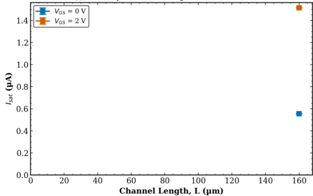
TFT2 Transistor 2 I_{sat} vs L | W = 1000 \mu\text{m} (mean \pm std)
