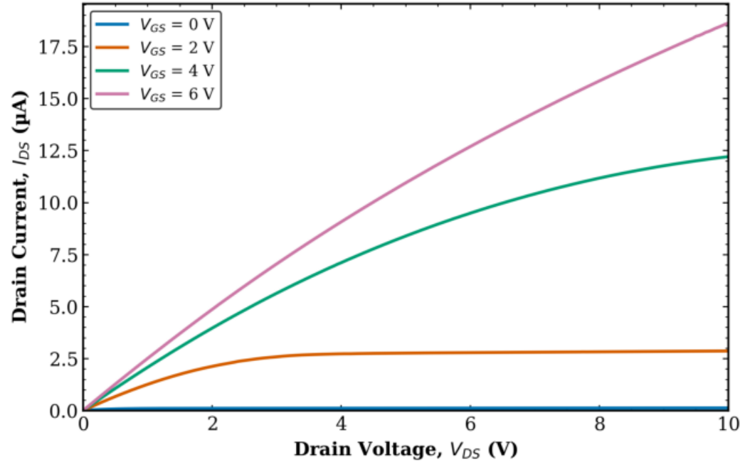
TFT2 Transistor 2 L = 160 \mu\text{m} , W = 500 \mu\text{m}
