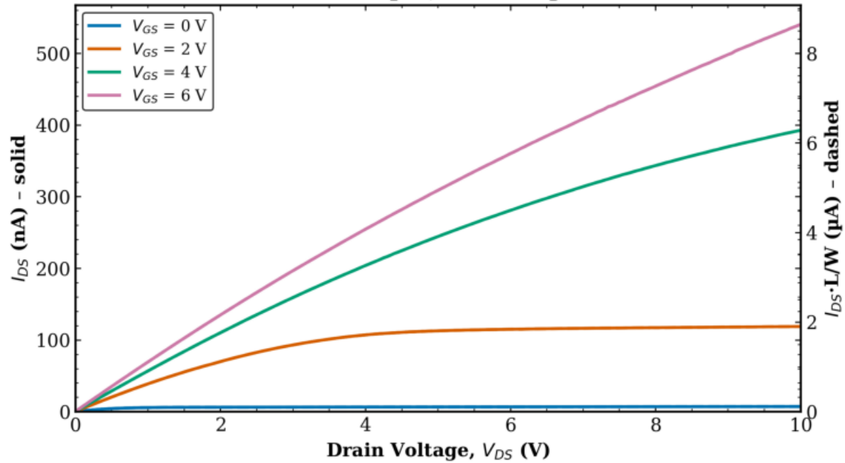
TFT2 Transistor 2 L = 160 \mu\text{m} , W = 10 \mu\text{m}
