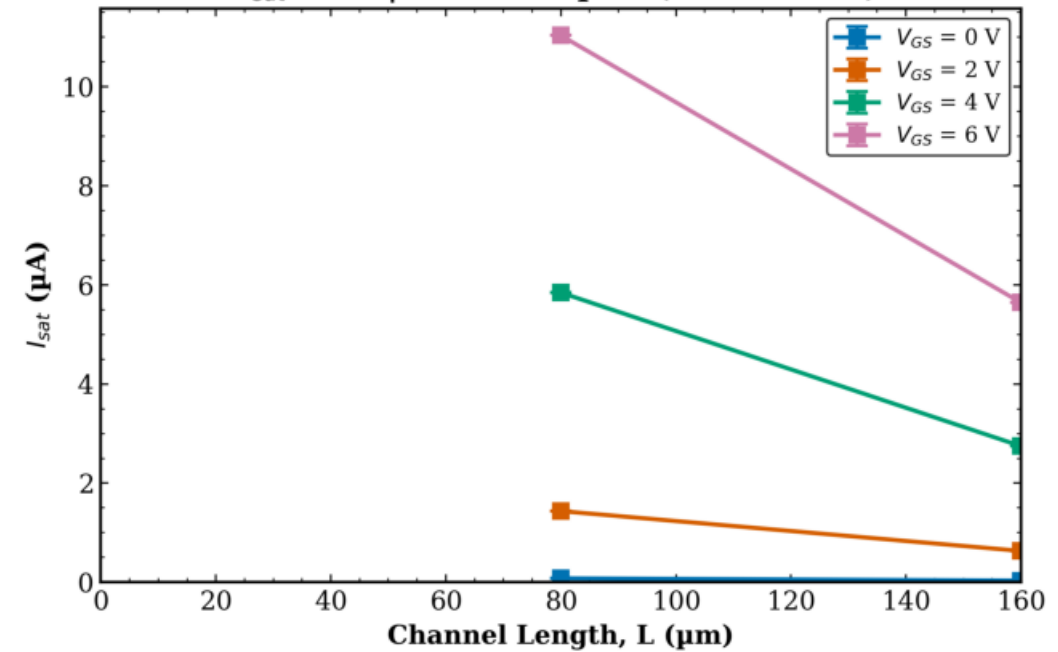
TFT2 Transistor 2 I_{sat} vs L | W = 100 \mu\text{m} (mean \pm std)
