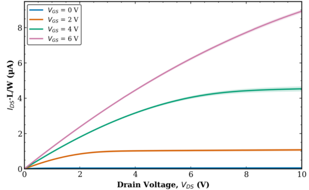
TFT2 Transistor 2 W = 100 \mu\text{m} - avg over all L (mean \pm std)
