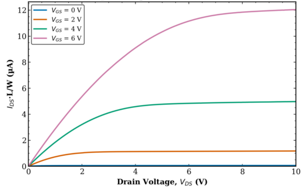
TFT2 Transistor 2 W = 50 \mu\text{m} - avg over all L (mean \pm std)
