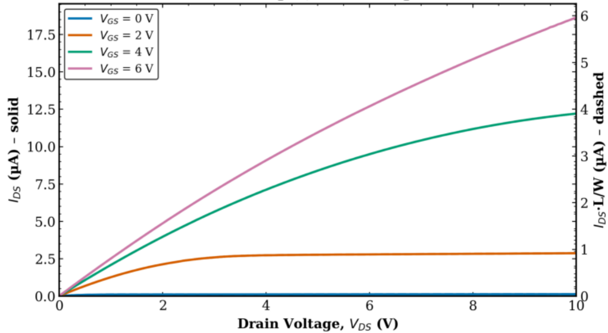
TFT2 Transistor 2 L = 160 \mu\text{m} , W = 500 \mu\text{m}
