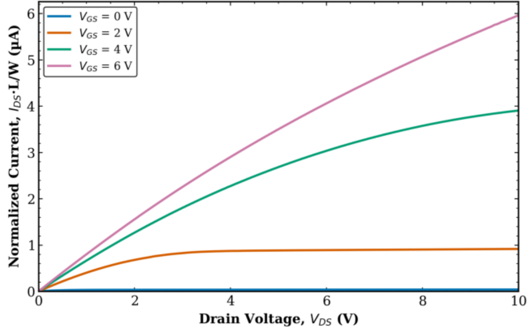
TFT2 Transistor 2 L = 160 \mu\text{m} , W = 500 \mu\text{m} (normalized)
