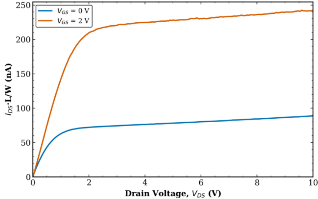
TFT2 Transistor 2 W = 1000 \mu\text{m} - avg over all L (mean \pm std)
