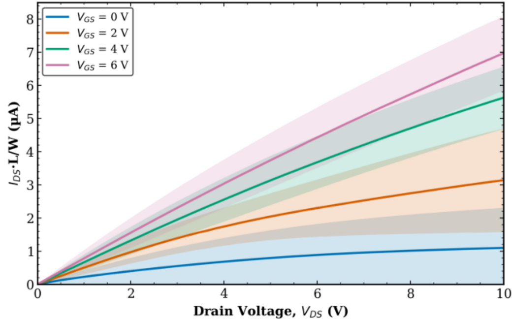
TFT2 Transistor 2 W = 10 \mu\text{m} - avg over all L (mean \pm std)
