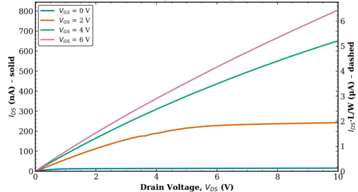
TFT2 Transistor 2 L = 80 \mu\text{m} , W = 10 \mu\text{m}
