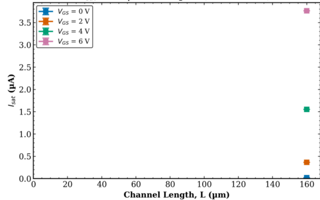
TFT2 Transistor 2 I_{sat} vs L | W = 50 \mu\text{m} (mean \pm std)
