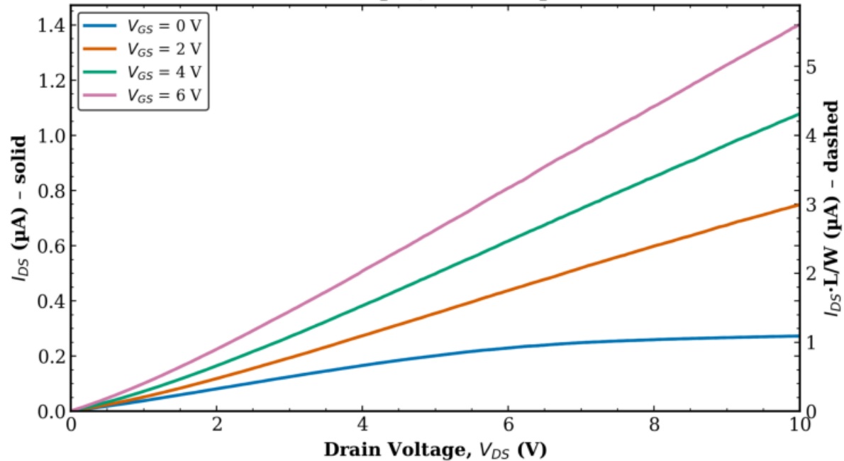
TFT2 Transistor 2 L = 40 \mu\text{m} , W = 10 \mu\text{m}
