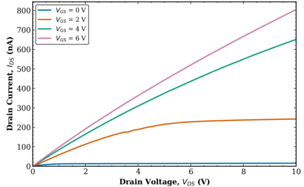
TFT2 Transistor 2 L = 80 \mu\text{m} , W = 10 \mu\text{m}
