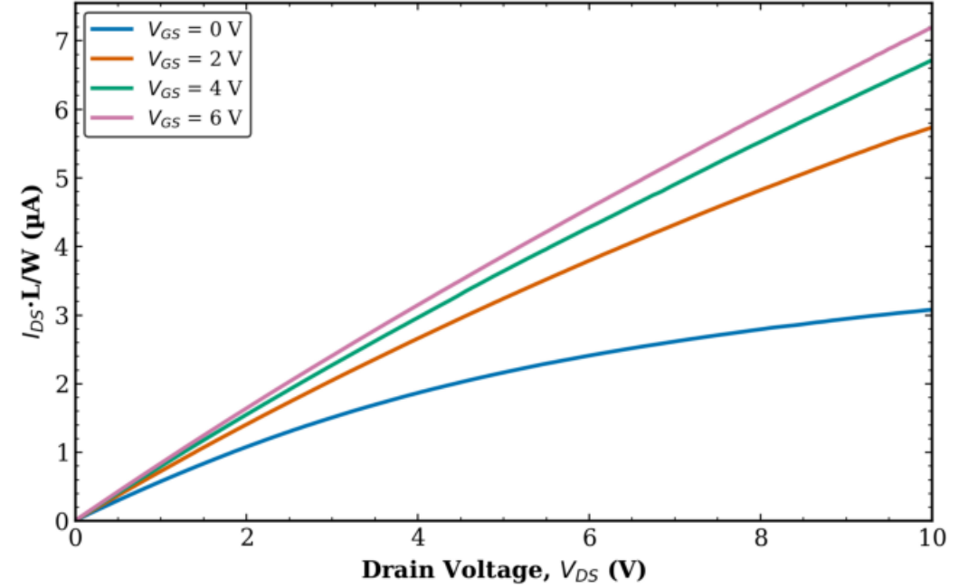
TFT2 Transistor 2 L = 20 \mu\text{m} - avg over all W (mean \pm std)
