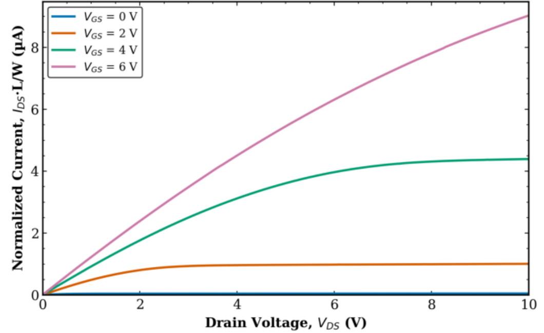
TFT2 Transistor 2 L = 160 \mu\text{m} , W = 100 \mu\text{m} (normalized)
