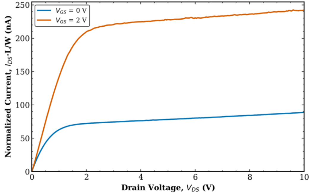
TFT2 Transistor 2 L = 160 \mu\text{m} , W = 1000 \mu\text{m} (normalized)
