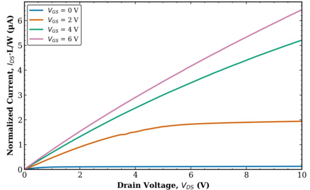
TFT2 Transistor 2 L = 80 \mu\text{m} , W = 10 \mu\text{m} (normalized)
