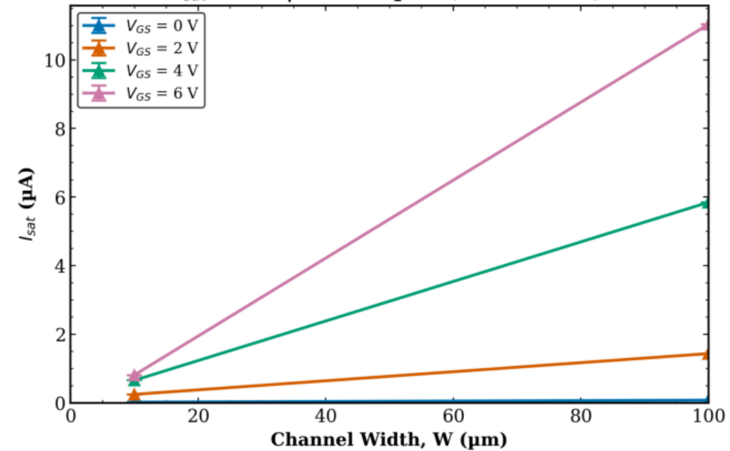
TFT2 Transistor 2 I_{sat} vs W | L = 80 \mu\text{m} (mean \pm std)
